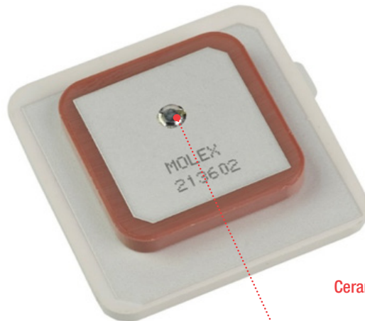
GPS L1/L2 36mm Stacked Patch Antenna (Series 213602)
