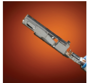
This Mini-Fit Plus HCS™ terminal has been crimped using the Molex TM-3000 press with a Molex applicator
