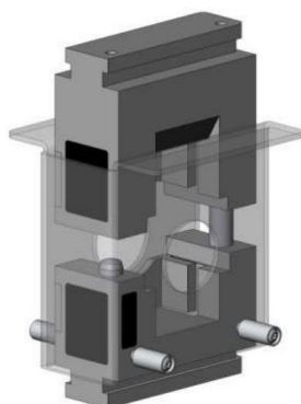
Crimp Adapter for DIN-Style Dies (63801-8901)
